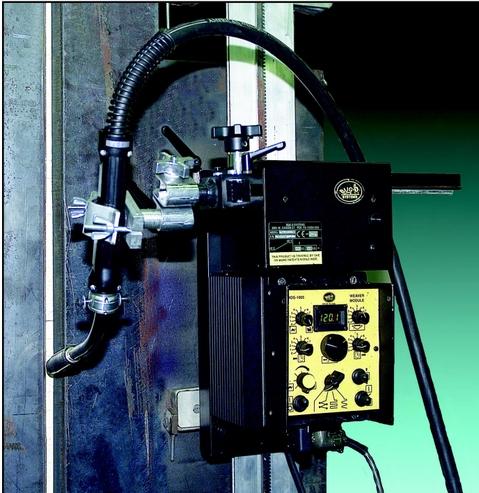
One-sided welding with Bug-O Systems MDS Travel Carriage.
